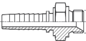
TE0115 PAG. BSPP MALE (60° CONE SEAT)
