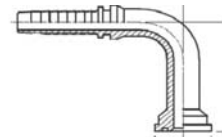
TE0114 PAG. BSPP FEMALE SWIVEL (60° CONE SEAT) - 90° ELBOW
