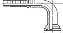
TE0113 PAG. BSPP FEMALE SWIVEL (60° CONE SEAT)
