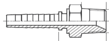
TE0117 PAG. BSPT TAPERED MALE (60° CONE SEAT)
