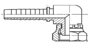
TE0116 PAG. BSPP FEMALE SWIVEL (60° CONE SEAT) - 90° ELBOW (COMPACT)
